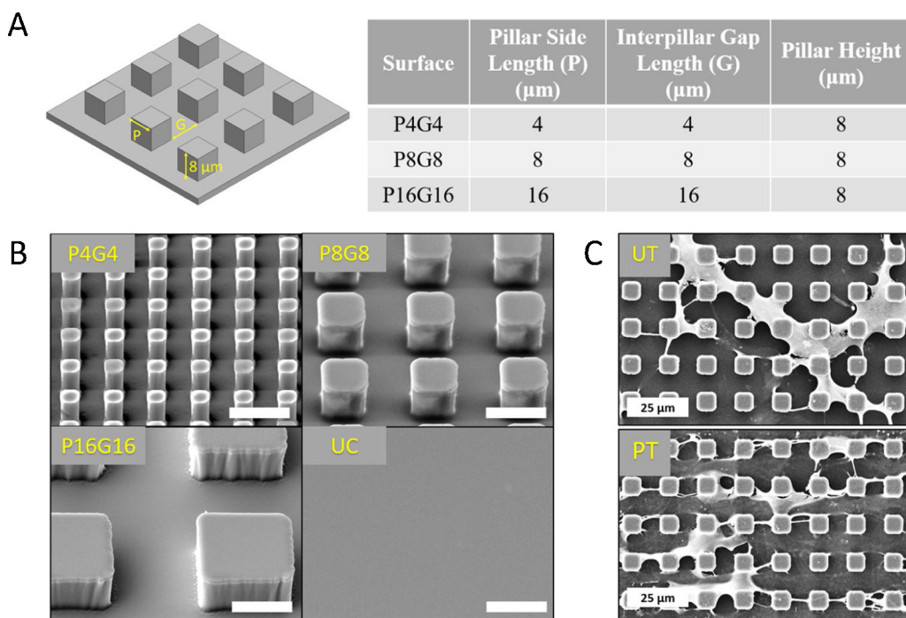
Fig. 1. Dimensions and images of the PMMA films. (A) Dimensions of the three PMMA surfaces decorated with square prism micropillars (P4G4, P8G8, P16,G16) and the unpatterned control (UC). (B) SEM micrographs of the micropatterned PMMA films. Scale bars: 10 μm. (C) Representative SEM micrographs of DPSCs on untreated (UT) and plasma treated (PT) P8G8 surfaces on Day 7.
