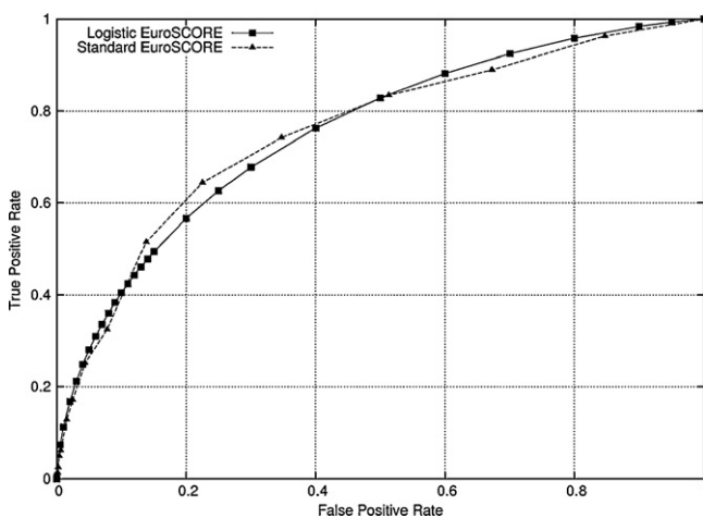
Fig. 1. Receiver operator curve of the additive and logistic EuroSCORE models for adult cardiac surgery analyzed from TurkoSCORE dataset ( n = 8018 ).
