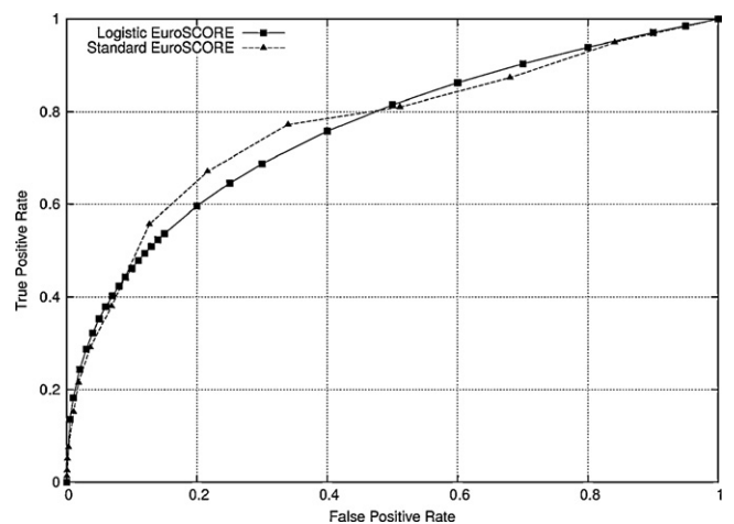
Fig. 2. Receiver operator curve of the additive and logistic EuroSCORE models for isolated CABG subset analyzed from TurkoSCORE dataset ( n = 6171 ).
