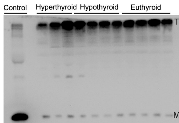
Fig. 5 Discrimination of monomeric (M) and tetrameric (T) transthyretin (TTR) in serum of patients with hyperthyroidism and patients with hypothyroid as well as euthyroid patients determined by immunoblotting under semi-denaturing conditions. Samples were diluted 1:50 with a sample buffer containing SDS but not 2-mercaptoethanol and were not heated. The control was a serum sample diluted 1:50 using a sample buffer with SDS and 2-mercaptoethanol and which was heated to 95°C for 5 min. Amounts of monomeric and tetrameric TTR were determined by densitometry.
