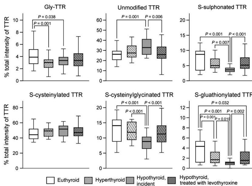
Fig. 4 Relative amounts (%) of unmodified TTR and TTR post-translationally modified at Cys 10 in serum of euthyroid patients as well as incident hyperthyroid patients, incident hypothyroid patients and hypothyroid patients with levothyroxine therapy determined by immunoprecipitation and subsequent MALDI-TOF-MS. Abbreviations used: Gly-TTR, TTR in which the cysteine side chain is chemically modified to form glycine; MALDI-TOF-MS, matrix-assisted laser desorption ionization-time of flight-mass spectrometry; TTR, transthyretin.
