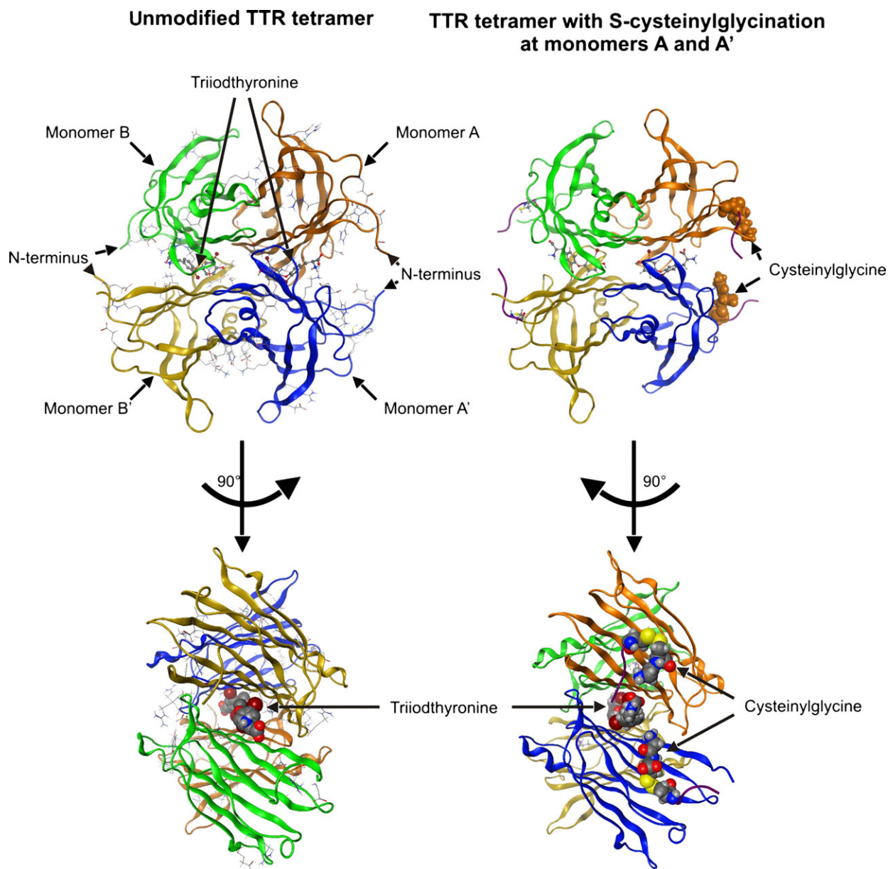
Fig. 1 Ribbon models of the transthyretin–triiodothyronine complex with unmodified Cys 10 and Cys 10 modified by S-cysteinylglycination in monomers A and A'. TTR is a tetramer composed of four identical subunits, which are annotated as monomer A (orange), monomer A' (blue), monomer B (green) and monomer B' (yellow). Monomers A and B associate to form a dimer, as do the monomers A' and B'. Subsequently, both dimers associate to form the tetramer. The thyroid hormone-binding cavities are located at the interface between the dimer units and their entrances are formed by the monomers AA' and BB' respectively [2, 3].
