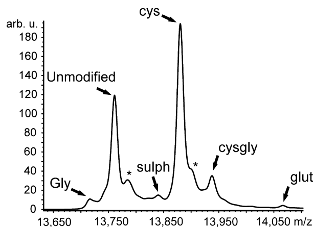
Fig. 3 MALDI-TOF mass spectrum of transthyretin (TTR) after immunoprecipitation from serum. According to the molecular weight, the TTR variants were assigned as follows: TTR in which the cysteine side chain is chemically modified to form glycine (Gly, 13,718 Da), unmodified TTR (13,762 Da), sulphated TTR (sulph, 13,841 Da), cysteinylated (cys, 13,881 Da), cysteinylglycinated TTR (cysgly, 13,938 Da), and glutathionylated TTR (glut, 14,067 Da) [11, 12, 26]. The asterisk indicates adducts with sodium (+22 Da).
