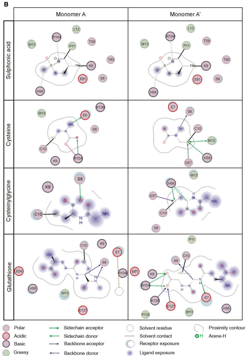
Fig. 2 Amino acid sequence of human transthyretin polypeptide chain and its interaction with different substituents of Cys 10 . Amino acid sequence in single letter code is shown in A and was adapted from [7]. Single underlined amino acids are residues in the core of the thyroid hormone-binding site and double underlined amino acid are residues within the central channel. Modification of Cys 10 influences binding characteristics of the tertiary structure and the magnitude of the effects depend on the chemotype of the substituent as well as the position of the modified monomer within the tetrameric structure (B).
