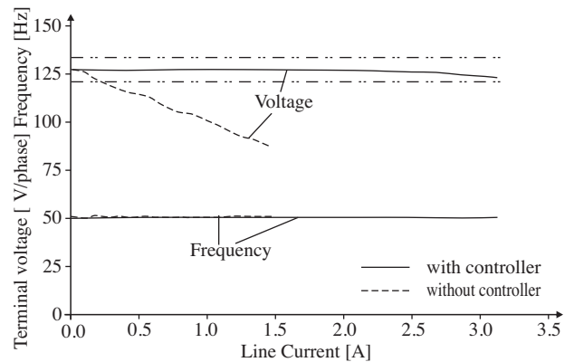
Figure 5. Steady-state performance of PVCEA under inductive load.
