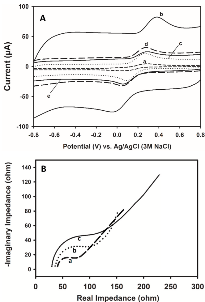
Fig. 2. A) Cyclic voltammograms of (a) GCE, (b) GO/GCE, (c) f-GO/GCE, (d) AB/f-GO/GCE and (e) BSA/AB/f-GO/GCE in 1 mM of K_3[Fe(CN)_6] and 1 mM of K_4[Fe(CN)_6] with a scan rate of 50 mV/s. B) EIS spectrum of (a) GO/GCE, (b) AB/f-GO/GCE and (c) BSA/AB/f-GO/GCE in 1 mM of K_3[Fe(CN)_6] , 1 mM of K_4[Fe(CN)_6] and 0.1 M of KCl between 50,000 and 0.5 Hz.
