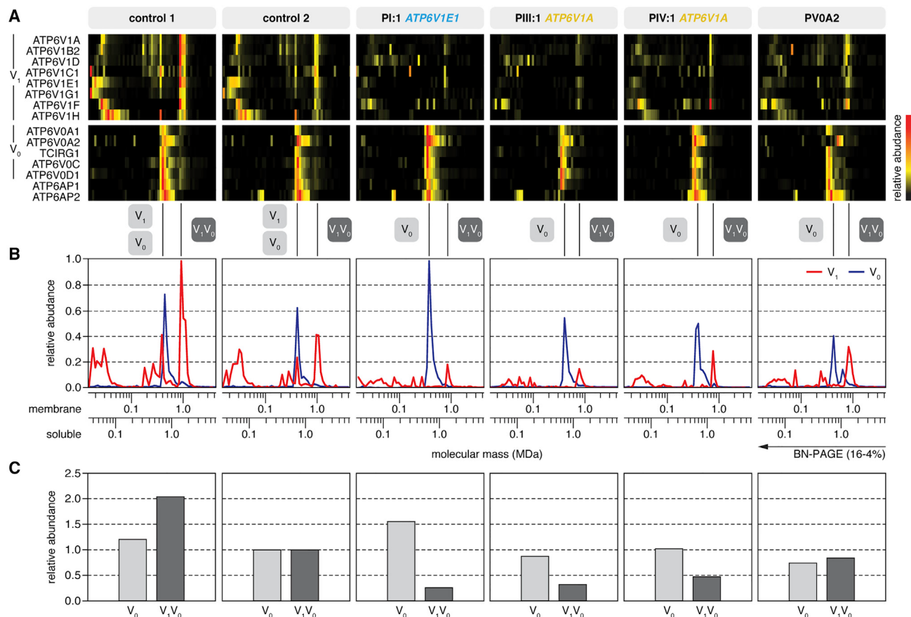
Figure 3. Complexome Profiling
